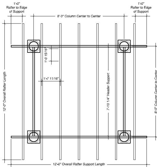
Rafter Supports & Rafters
