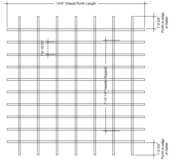
Rafters & Purlins
